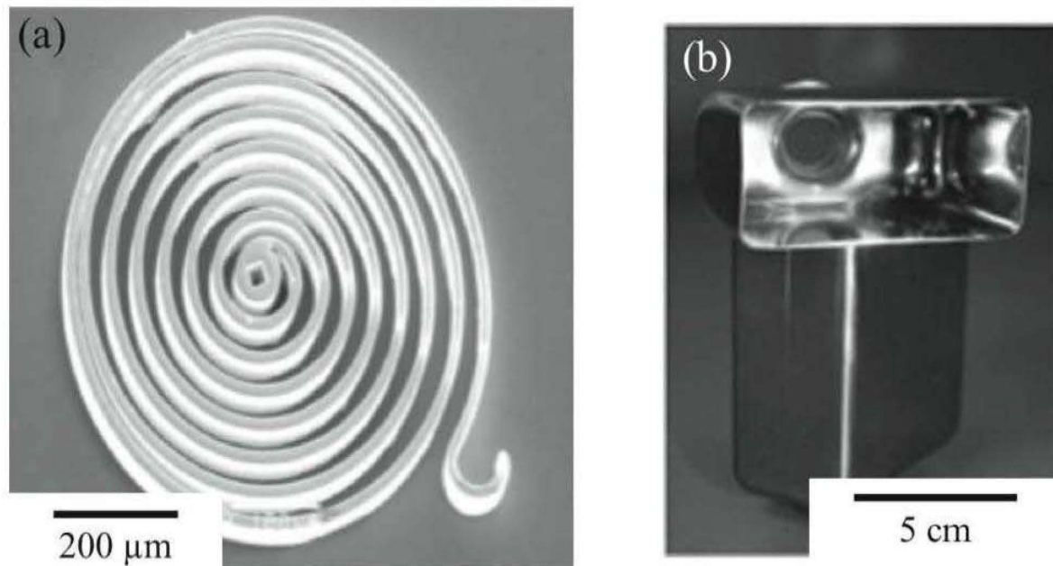
Figure 3. Examples of Processing of Metallic Glasses. (a) Microspring produced by lithography and (b) thin-walled bottle produced by blow molding. Images are courtesy of Professor Jan Schroers (Yale University).
