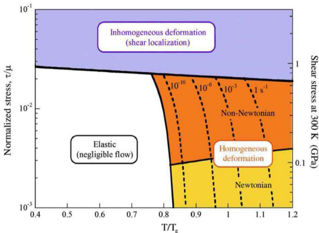
Figure 6. Deformation Map for Metallic Glasses. As a function of temperature (normalized to the glass transition temperature) and applied shear stress \tau (normalized to the shear modulus, \mu ). At high stresses, plastic deformation occurs inhomogeneously, being localized into shear bands. At high temperatures, plastic deformation becomes homogeneous. The dashed lines represent different strain rates. The absolute stresses given are representative of the well-studied bulk metallic glass Zr 41.2 Ti 13.8 Cu 12.5 Ni 10 Be 22.5 , but the general features of the map are expected to apply to all metallic glasses. 23
