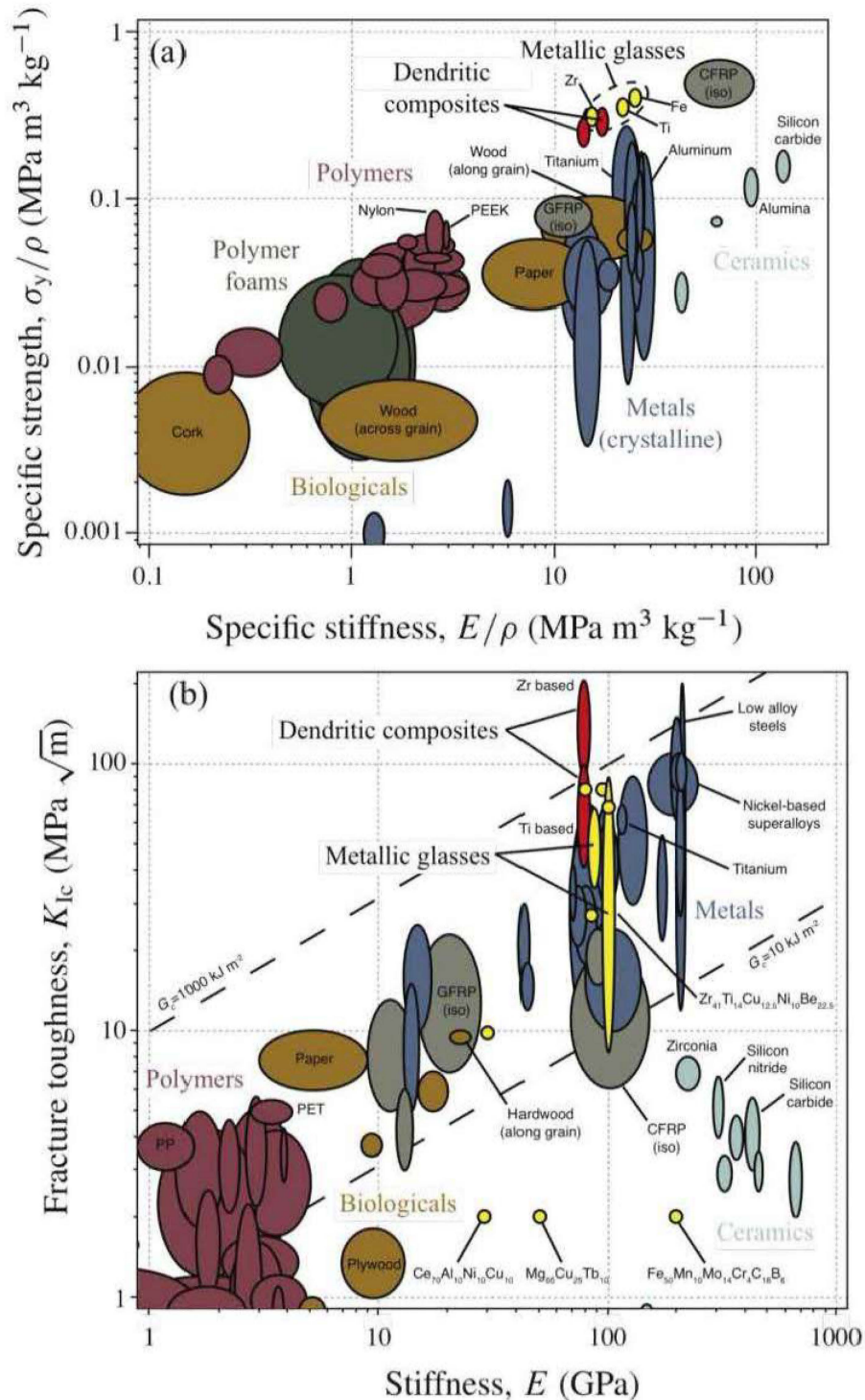
Figure 9. Materials Property Charts. (a) Strength and stiffness (both normalized to density) of metallic glasses (yellow) and dendritic metallic glass matrix composites (red) compared with other materials. (b) Damage tolerance. On this plot, the dashed lines represent contours of equal fracture energy. In both plots, polymer composites (CFRP and GFRP) are represented by isotropic averages; continuous fiber composites can have greater strength and stiffness in a direction parallel to the fibers. 39
