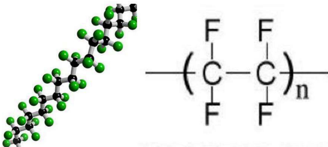
Figure 8. Teflon Structure
