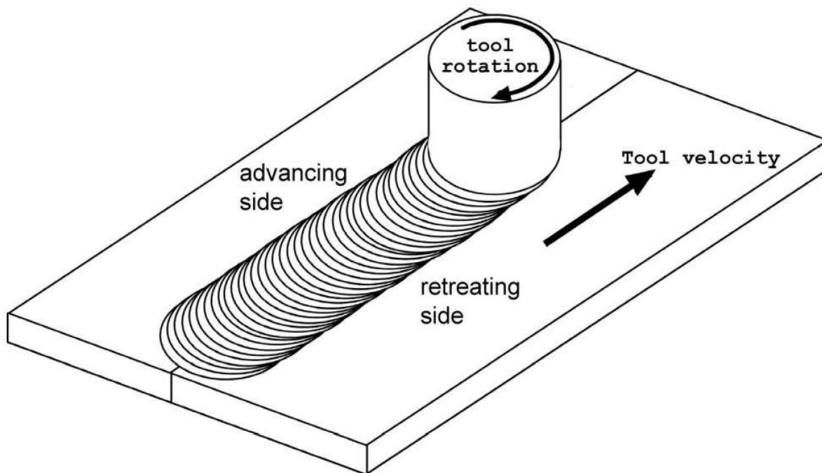
Figure 1. Schematic Diagram of Friction Stir Welding
