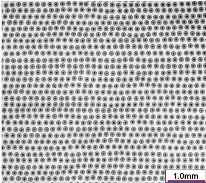
Figure 4. Cross-Section Micrograph of a Ti Matrix Composite. Small, dark centers of fibers are C monofilament substrates for deposition of SiC (light micrograph). Material system: Matrix alloy – Ti-6242; Fiber – SiC about 5.6-mil-diameter SCS-6
