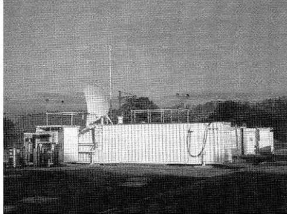
Figure 3. Orion HPM Testing Facility
