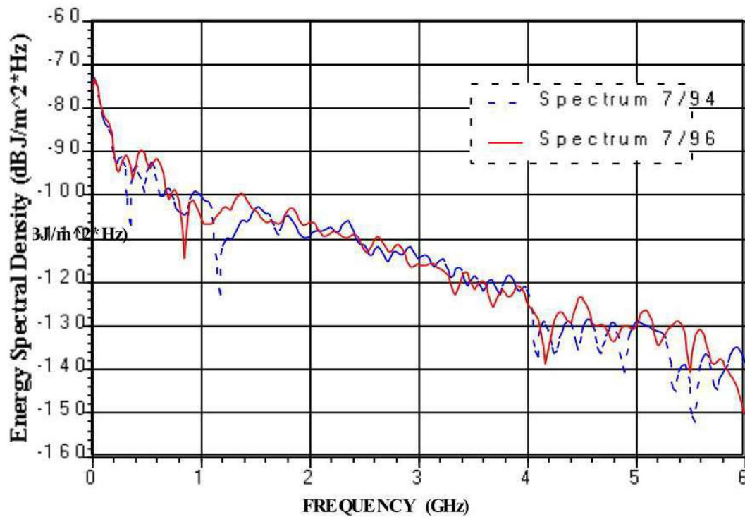
Figure 9. Phoenix Radiated Spectral Content
