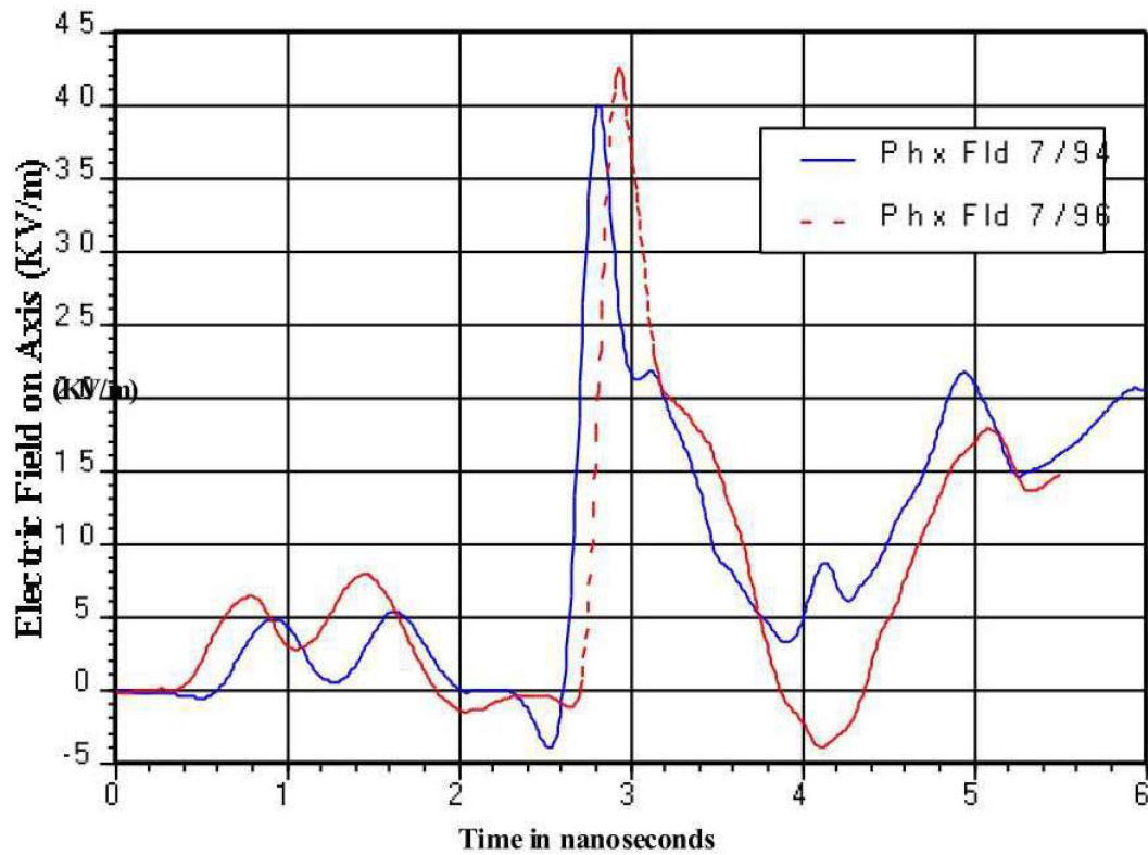
Figure 8. Phoenix Radiated Pulse at 8.5 Meters
