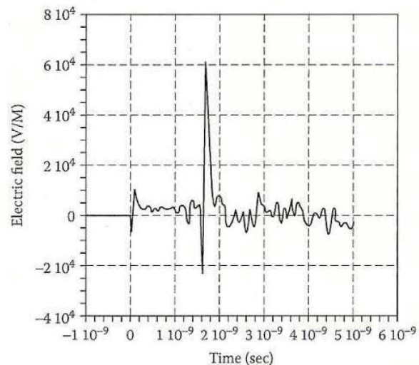
Figure 11. Jolt Radiated Electric Field Waveform at 85 Meters
