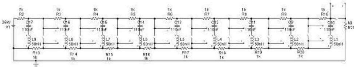
Figure 2. Example of Marx Generator Circuit
