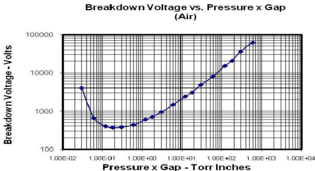
Figure 1. Paschen Curve for Air
