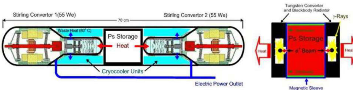
Figure 15. Conceptual 110-Watt Positron Closed-Cycle Generator Based on the NASA Glenn Research Center Stirling Radioisotope Generator 47 (courtesy Positronics Research LLC) 48
