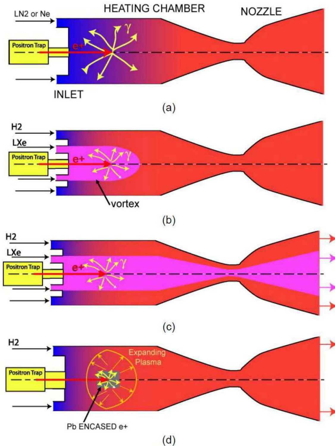
Figure 12. Fluid Systems. (a) One-fluid system of \text{LN}_2 or Ne propellant; (b) Two-fluid system of \text{LH}_2 and \text{LXe} ; (c) Two-fluid flow-through system with \text{LH}_2 at higher mass flow rates than \text{LXe} ; and (d) One-fluid \text{LH}_2 system with lead encapsulated Ps (courtesy Positronics Research LLC) 36
