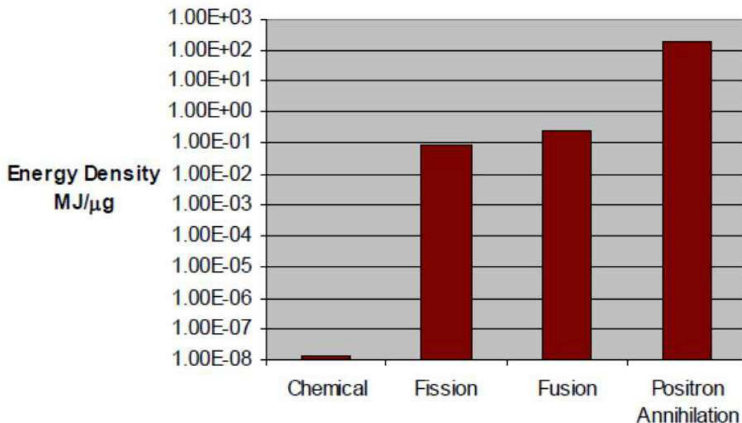
Figure 1. Specific Energy for Chemical, Nuclear, and Antimatter Materials
