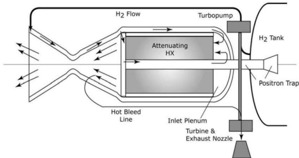
Figure 11. Solid-Core Positron Rocket Engine With a Hot-Bleed Configuration (courtesy Positronics Research LLC) 30
