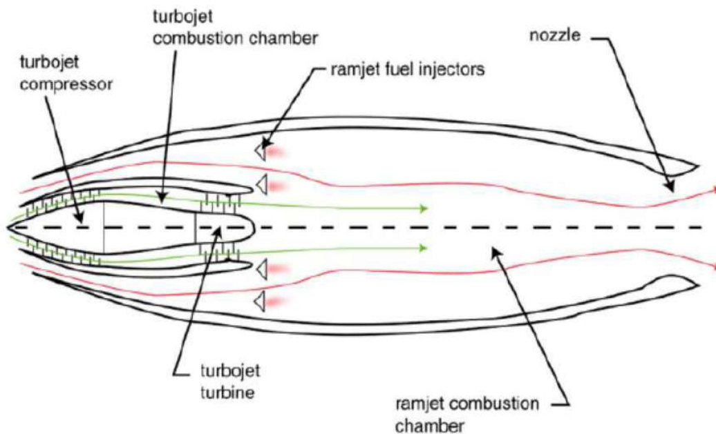
Figure 5. Combustion Turbo-Ramjet (courtesy Positronics Research LLC) 13
