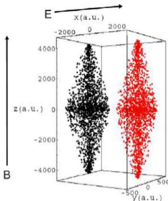
Figure 21. Computer Simulation of Ps Atoms in a 5-Tesla Magnetic Field and 100 V/cm Electric Field (1 a.u. = 0.052 nm) (courtesy University of Bielefeld, Germany) 74
