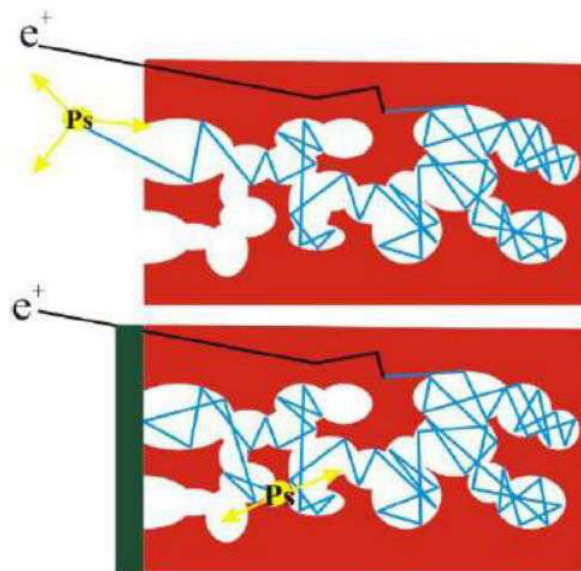
Figure 20. A Positron Forms Ps on the Edge of a Void, Thermalizes, and Becomes Trapped in a Void Before Annihilating (courtesy University of Michigan)
