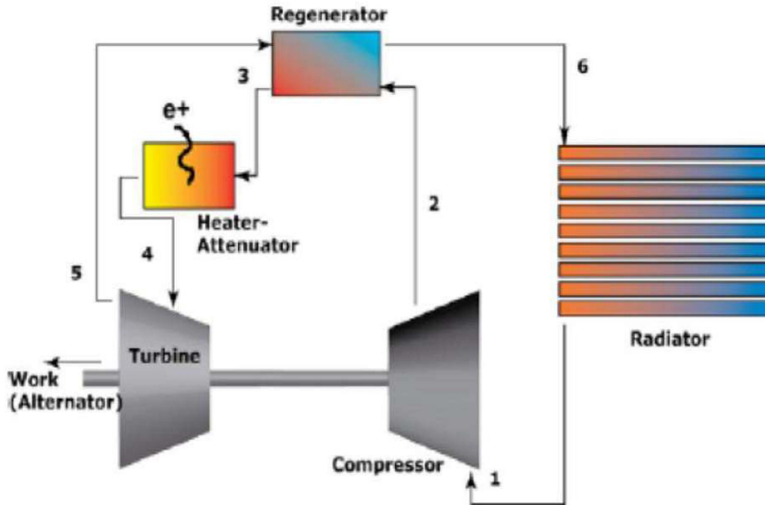
Figure 14. Closed Brayton Cycle Using Positron Annihilation (courtesy Positronics Research LLC) 45
