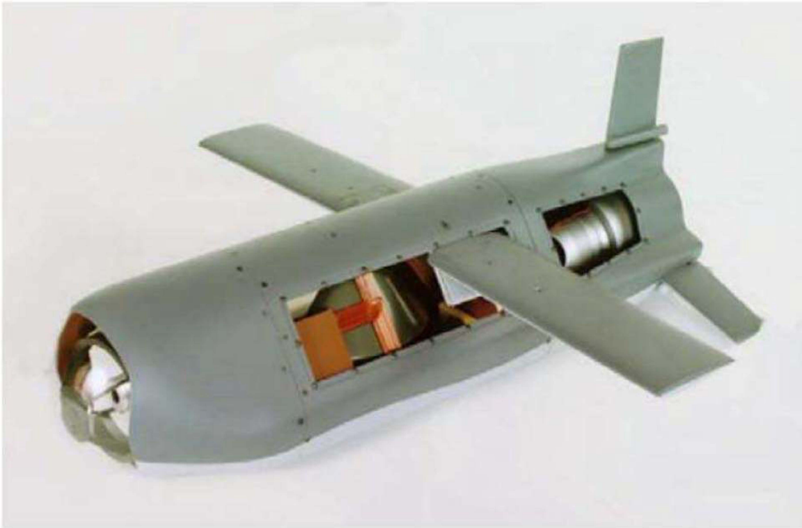
Figure 7. LOCAAS Turbojet Engine (courtesy of AFRL, Eglin AFB, FL) 17
