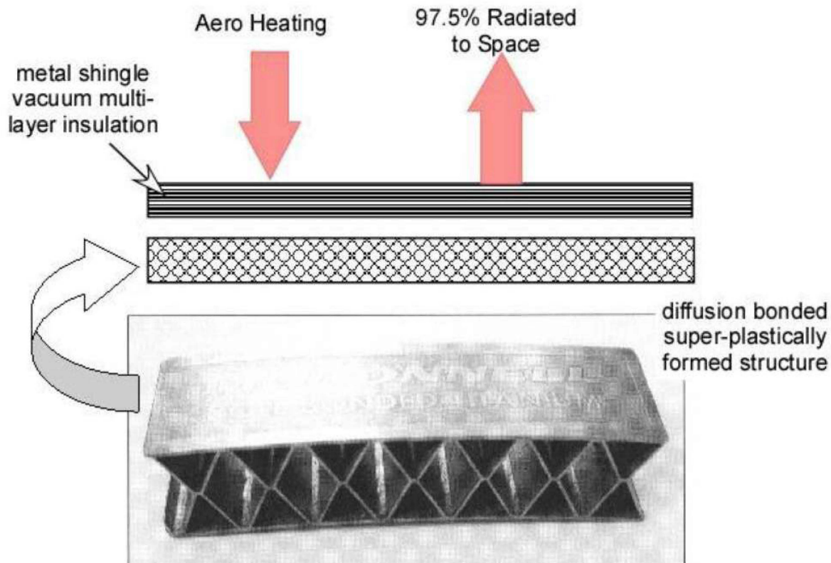
Figure 6.1 McDonnell titanium structure. (Courtesy of John Robson)
