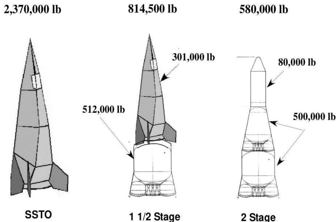
Figure 35. Propellant Tanks That Are Not Reentry Vehicles Greatly Reduce System Weight. Venture star orbital maneuver rules.
