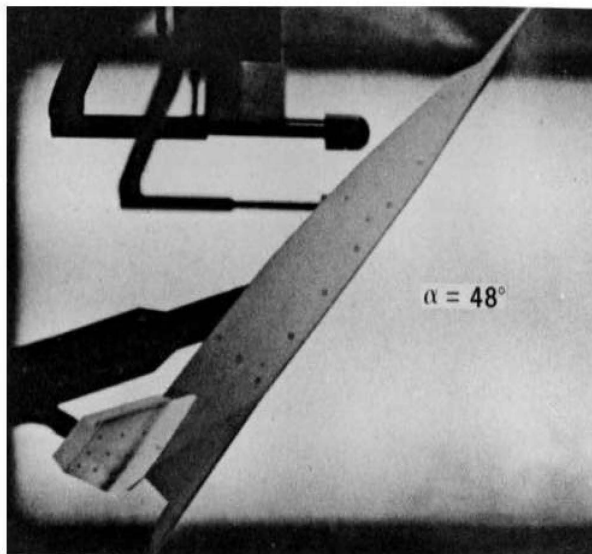
Figure 20. Thermographic Phosphor Image of Model 176 at Near-Maximum Angle of Attack
