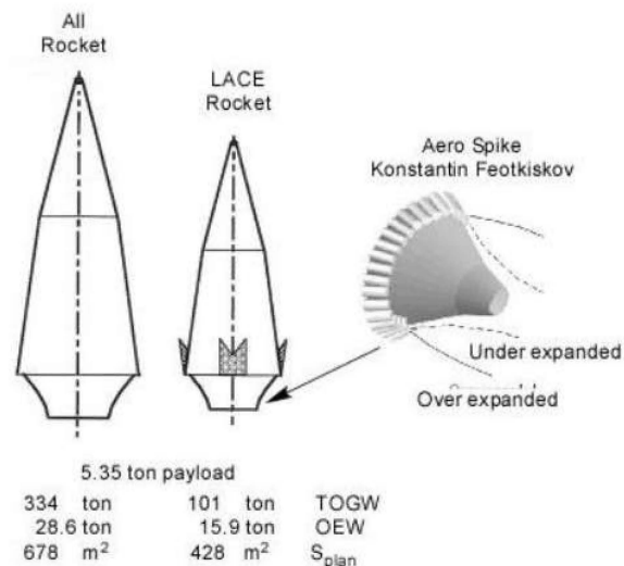
Figure 2. Impact of Air-Breathing Rocket
