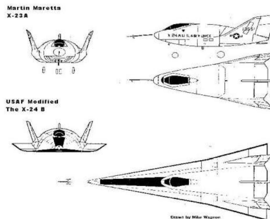
Figure 6. Martin Marietta X-24 A & B Research Gliders. X-24A based on USAF PRIME configuration.
