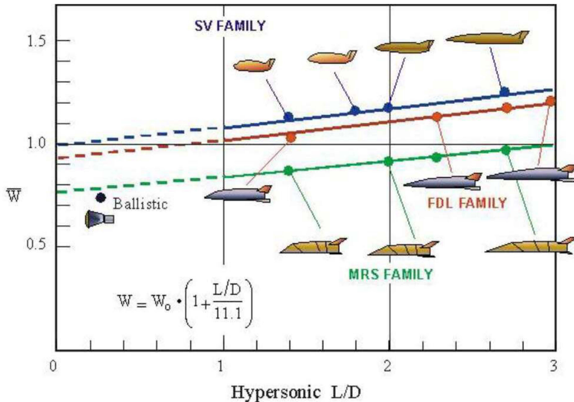
Figure 7. Detailed Design Analyses Show the Weight Trends are as Much a Function of Configuration Family as Lift-to-Drag Ratio
