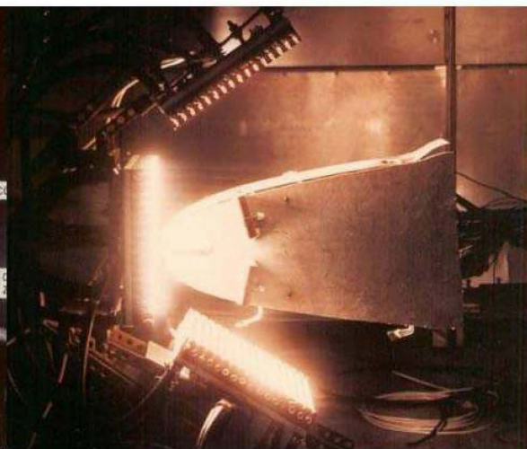
Figure 26. Heat Pipe Shuttle Leading Edge Designed and Built by McDonnell Douglas Astronautics. Tested extensively at McDonnell Douglas Corporation, St. Louis, and NASA Langley, it never failed.
