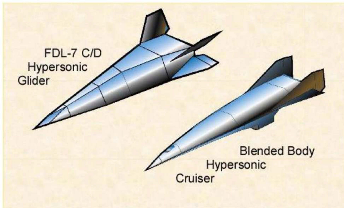
Figure 8. High-Performance Hypersonic Glide Aircraft. Rocket boost-glide and air-breather cruiser.
