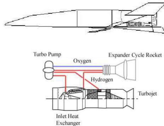
Figure 32. The FDL-7 Class of Vehicles With An Anthony DuPont Variable Capture and a Retractable Inlet Tested to Mach 5 Employing an Air-Breathing KLIN Cycle Rocket
