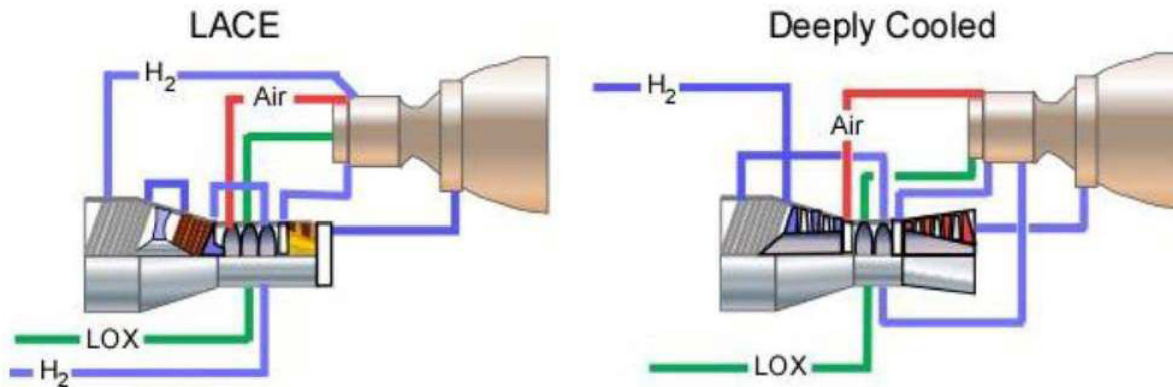
Figure 29. Two Rocket Air-Breathing Rocket Cycles to Mach 5.5. To the left is one employing liquefied air (LACE cycle). To the right is one employing high-pressure air cooled to near saturation.
