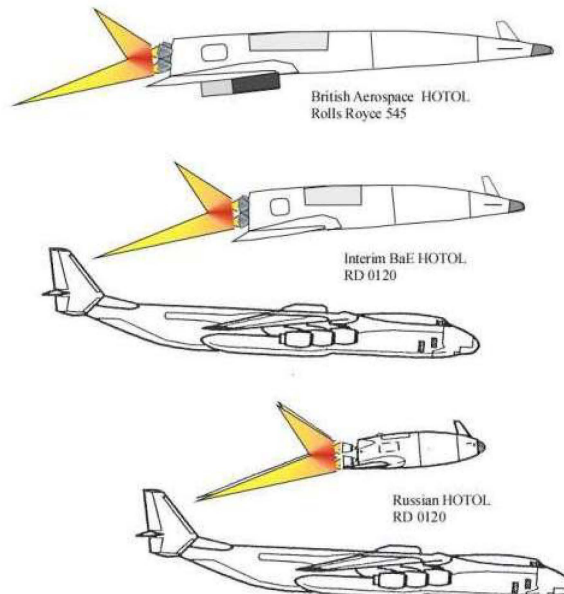
Figure 30. HOTOL Evolution: From Aerodynamic Optimum Configuration to Practical Launcher Configuration. The latter was developed through British Aerospace-Russian cooperation.
