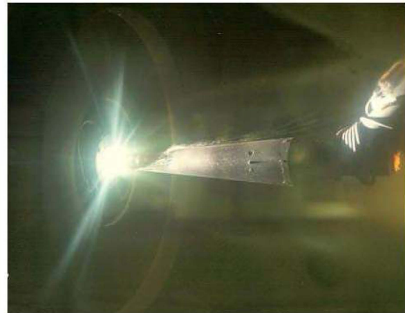
Figure 24. A Porous Nickel Tip Oozing Water. This test lasted 4,300 seconds before the arc heater cathode—not the nose tip—failed.
