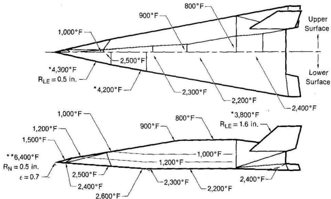
Figure 18. FDL-7C/D, Model 176 Entry Temperature Distribution. Upper-surface heating is minimized by cross-section geometry.
