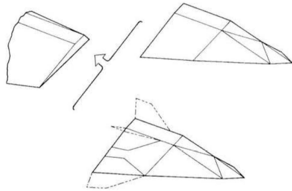
Figure 41. The FDL-7 and Model 176 Class of Hypersonic Gliders. The FDL-7 and Model 176 class of hypersonic gliders had integral, stable, controllable hypersonic-capable escape craft.
