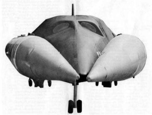
Figure 40. FDL-5 Scale Model of a Stage and One-Half Depicted 29
