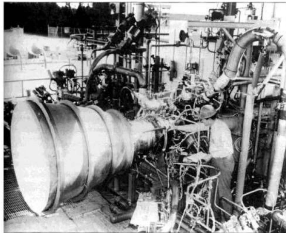
Figure 8.4 The XLR129 on the E8 test stand. (Courtesy of Pratt & Whitney)
