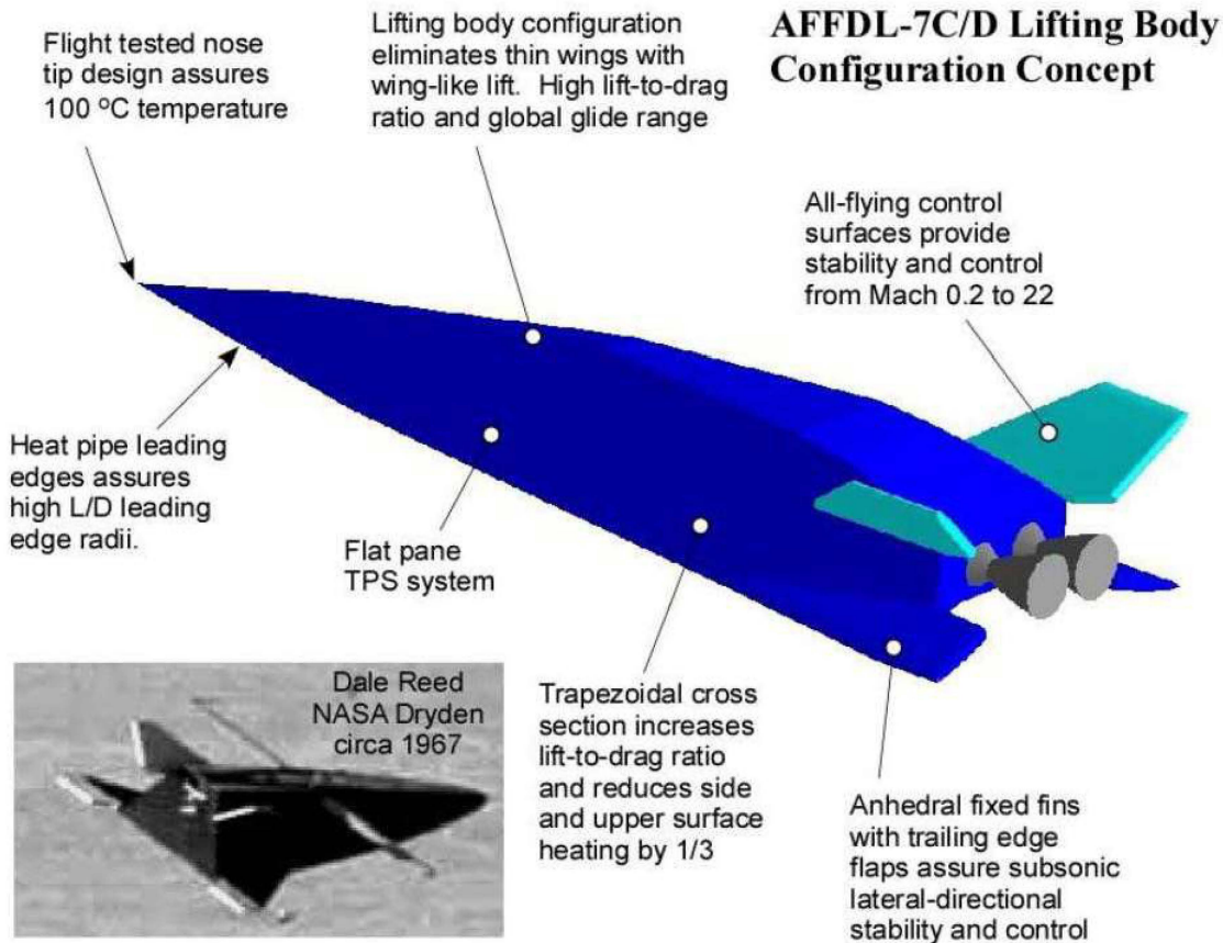
Figure 10. FDL-7C/D and FDL-7MC Lifting-Body Configuration. Offers inherent stability and control with sufficient volume and high lift-to-drag ratio.
