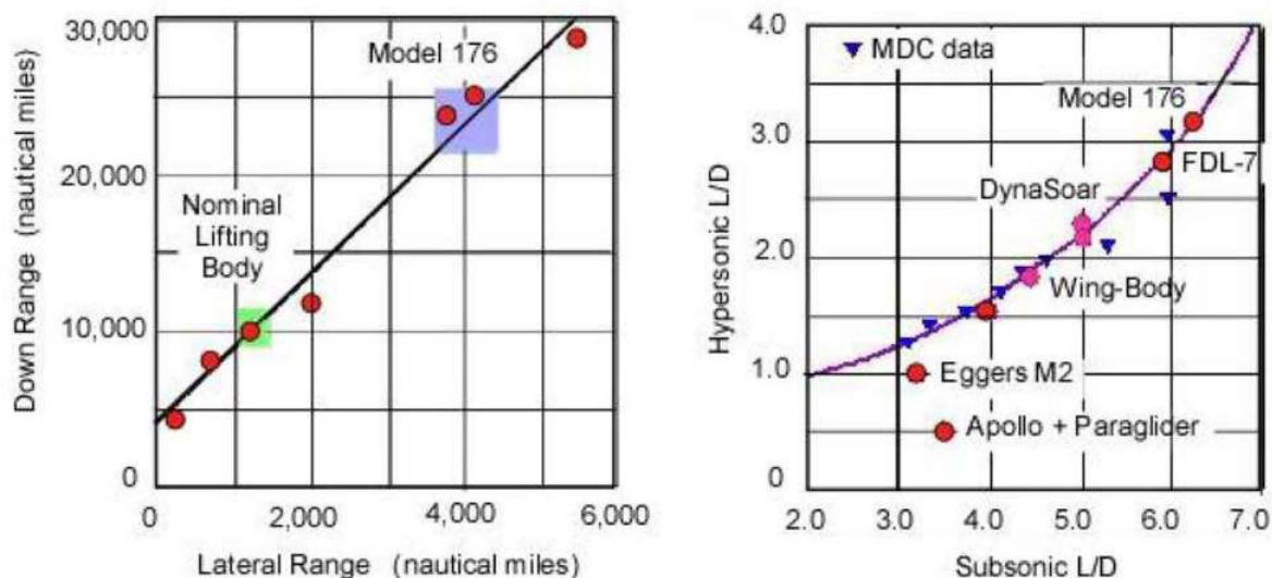
Figure 14. Hypersonic Glider Characteristics
