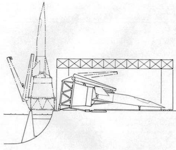
Figure 36. Simple Horizontal Integration and Vertical Launch Provides Rapid Launch Capability
