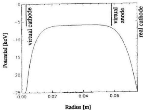
Figure 4.7. The Double Well Potential Calculated With IXL Code for d_{33\text{perp}} , i=14\text{keV} , I_i=55\text{A} , I_e=59\text{A}
