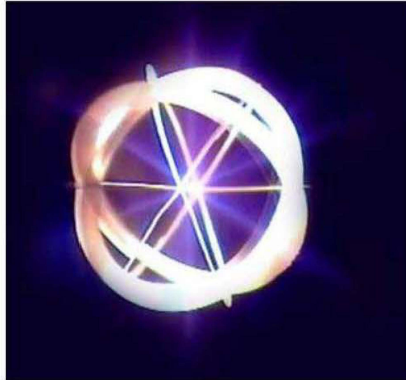
Figure 2.3. Photograph of a STAR mode discharge. The "vane" type grid shown is only one of a number of large opening grids designed and used for STAR mode operation of the neutron source type IEC. This particular design (but with variations) has been used by the UIUC, Daimler-Chrysler and Kyoto University. It is rugged, shows little sputtering and has proven very efficient for neutron production. Materials used vary from stainless steel to Mo.
