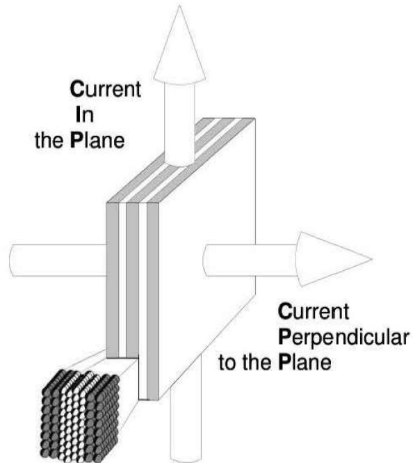
Figure 1. In a Magnetic Multilayer, Several Atomic Layers of Magnetic Material (shown in grey) Alternate With Layers of Nonmagnetic Material (shown in white). GMR occurs in one of two different geometries: (1) when the current flows in the plane (CIP geometry) of the layers or (2) when the current flows perpendicular (CPP geometry) to the layers.
