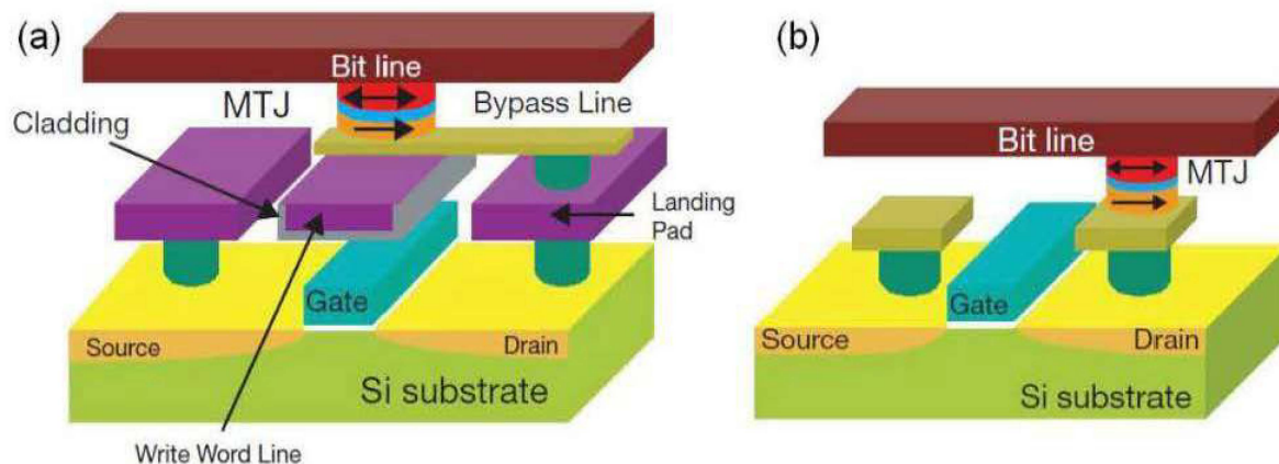
Figure 10. Conventional MRAM Cell (a) Versus STT MRAM Cell (b) (Reference 58)
