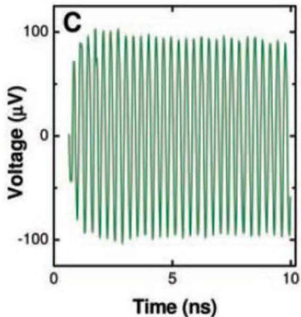
Figure 8. Oscillatory Voltage Generated by Precessional Motion of the Free Magnet in IrMn8nm/NiFe4nm/Cu8nm/NiFe4nm Nanopillar, in Response to a 335-mV dc Voltage Step Applied to the Device at B = 630 Oersteds (Reference 51)
