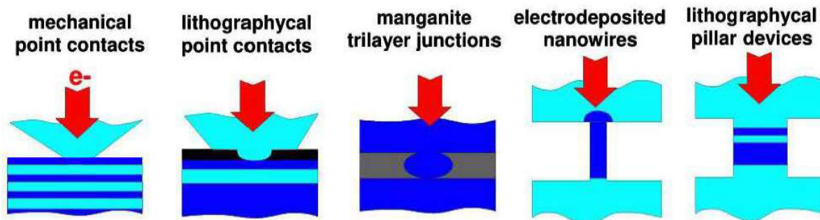
Figure 4. Device Schematics for STT Experiments. All experiments share one common feature: a small constriction for electrical current—that is, point contact, junction, nanowire, or nanopillar. Black (grey) indicates insulator; dark blue indicates magnetic material.
