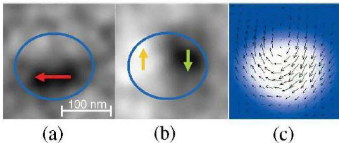
Figure 9. Scanning transmission x-ray microscopy images of M_x (a) and M_y (b) components of magnetization M combine into the vector field (c), which represents the direction of M in the plane of the CoFe free layer. (Reference 52)
