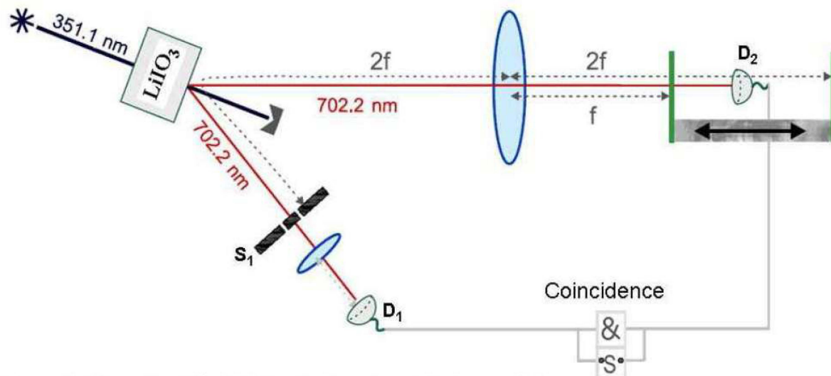
Figure 5. Schematic of the 1998 Dopfer Experiment (Reference 17)
