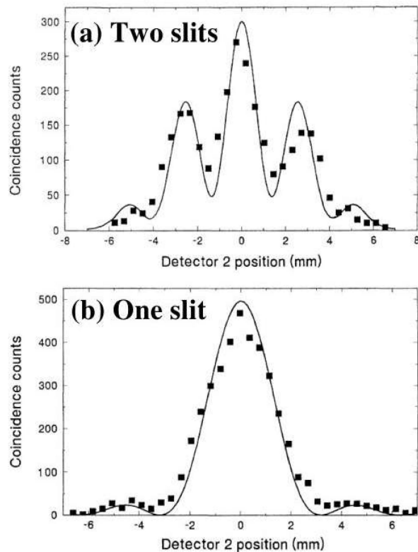
Figure 3. Ghost Interference Position Distributions at X_2
