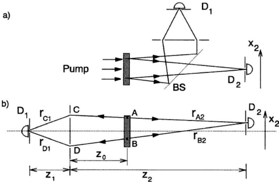
Figure 4. "Unfolding" the Ghost Interference Experiment
