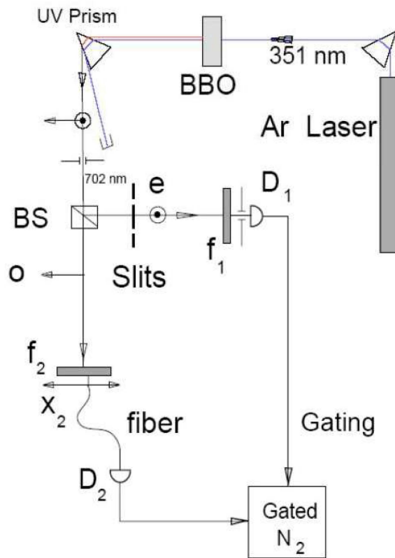
Figure 2. Schematic of the 1995 Ghost Interference Experiment (Reference 16) of the Shih group
