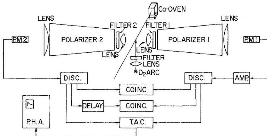
Figure 1. Schematic of the 1972 Freedman-Clauser Experiment (Reference 1)
