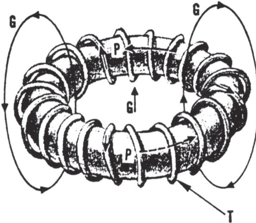
Figure 2. Dipole Gravitational Field Generator (Reference 14)
