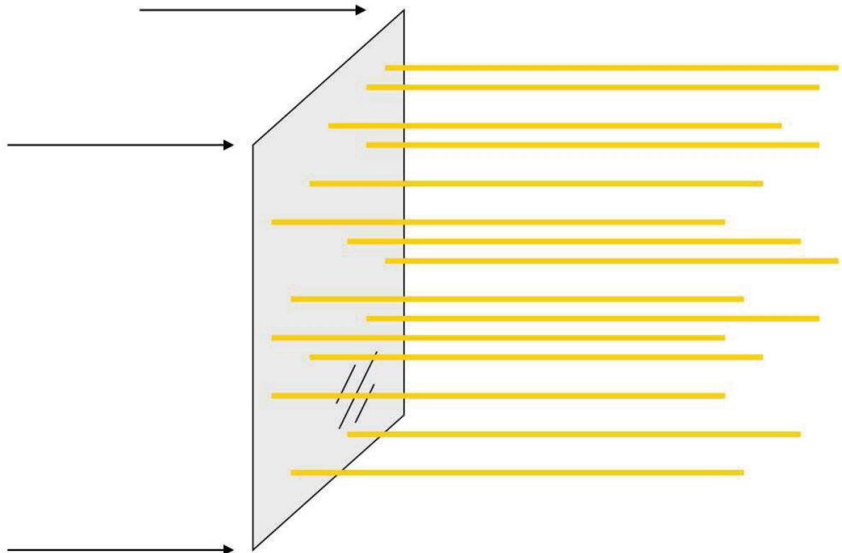
Figure 5. Negative Energy Flux (Gold) Emanating From a Moving Mirror
