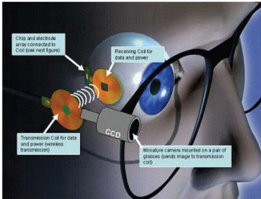
Figure 27. Power Transfer by Magnetic Induction to an Implanted BioMEMS Retinal Prosthesis. This is the Boston Retinal Implant Project.
