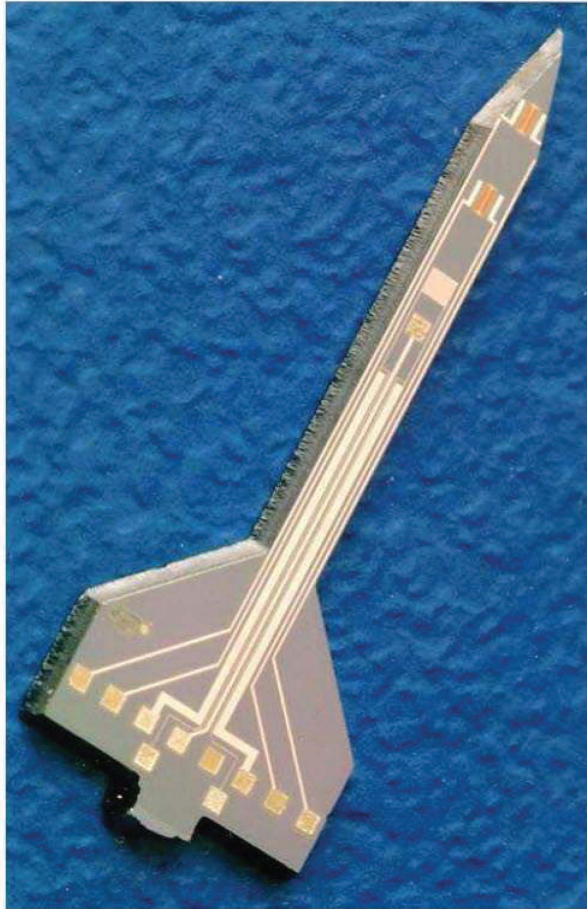
Figure 7. An ISFET (Ion Sensitive Field Effect Transistor) Needle-Type pH Sensor for Monitoring Tissue Physiologic Status ( http://www.ee.seikei.ac.jp/~seiichi/lecture/Biomedical/09/09-biosensor.html )
