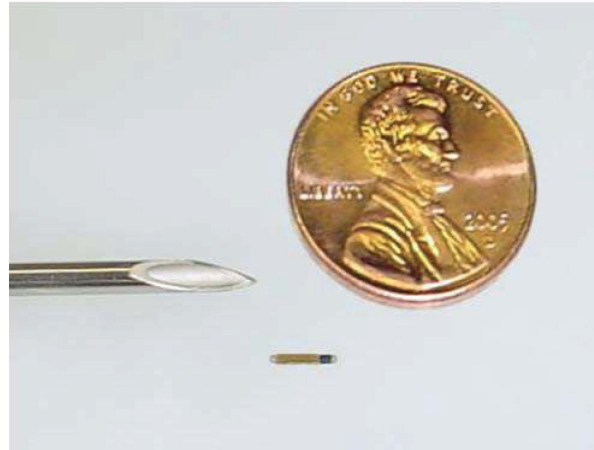
Figure 28. A New Generation of Implantable Neurostimulation Devices Can Pass Through the Lumen of a Syringe Needle. This device was made at ASU and is powered by ultrasound energy. (Towe et al.)
