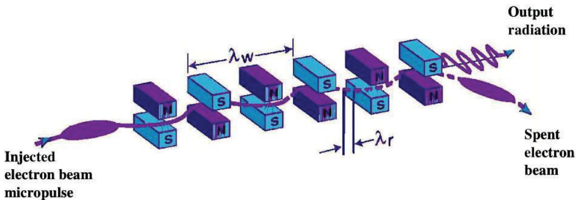
Figure 8. Free-Electron Laser Wiggler
