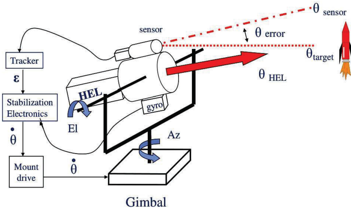
Figure 10. HEL Weapon Basic Tracking and Pointing Controls
