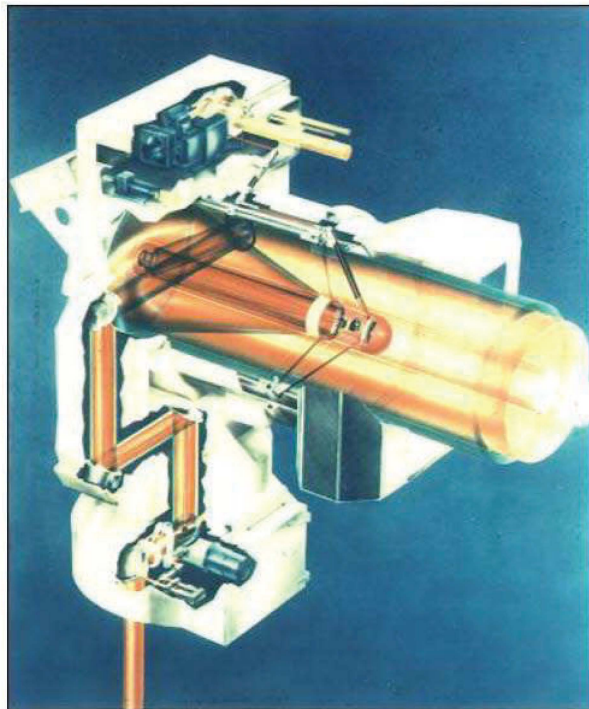
Figure 11. SeaLite Beam Director
