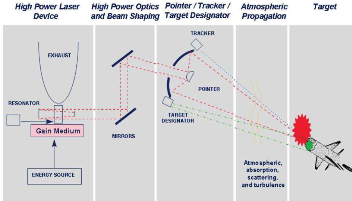
Figure 2. Elements of an HEL Weapon System
