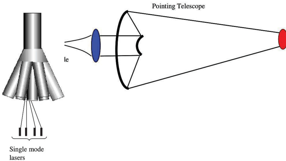
Figure 7. Incoherent Combination of Single Mode Lasers in a Fiber Combiner
