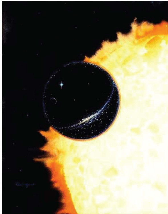
Figure 6. A Spherically Symmetric Traversable Wormhole Observed in Space
