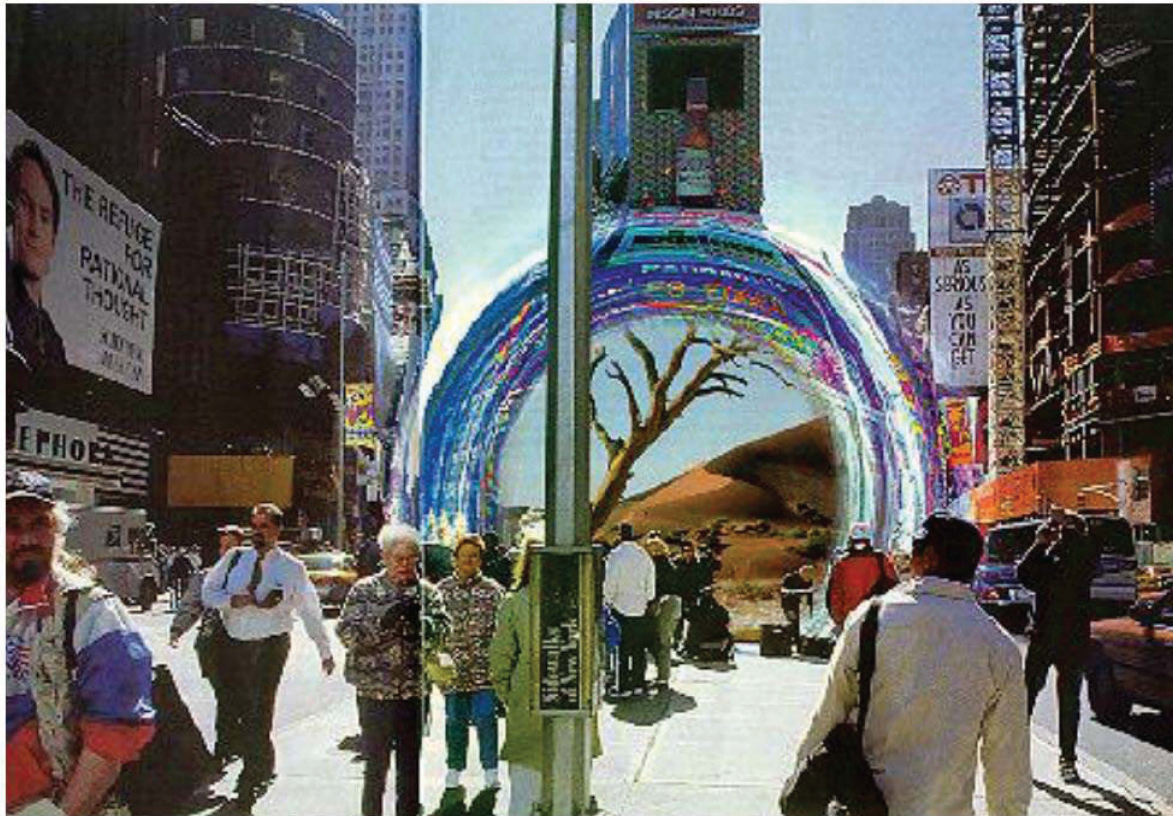
Figure 8. A Stargate in Times Square
