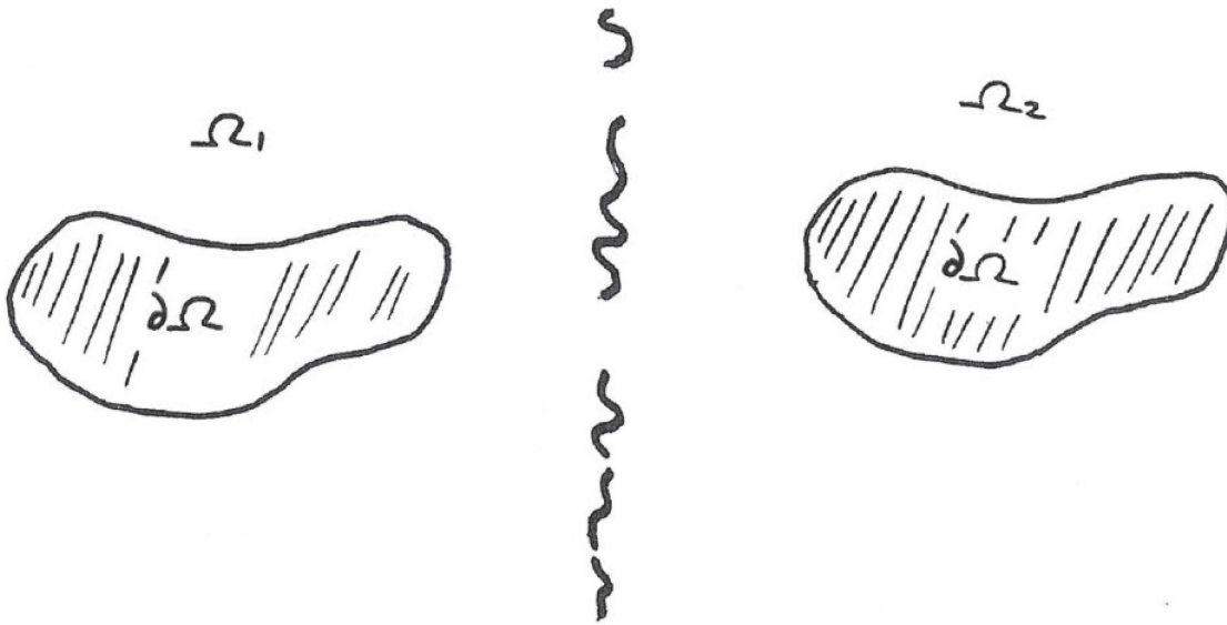
Figure 3. Diagram of a Simultaneous View of Two Remote Compact Regions, \Omega_1 and \Omega_2 , of Minkowski Space Used to Create the Wormhole Throat \partial\Omega (time is suppressed in this diagram)
