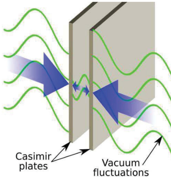
Figure 12. Schematic of the Casimir Effect
