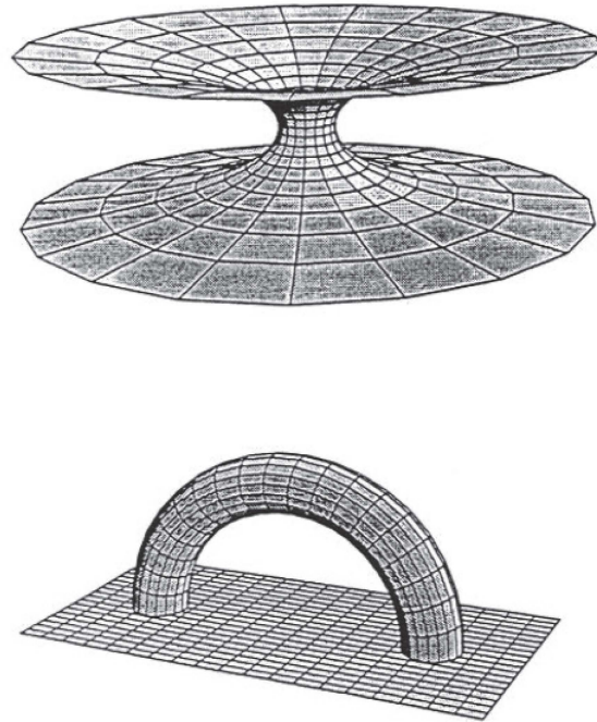
Figure 2. Inter-Universe Wormhole (top) and Intra-Universe Wormhole (bottom).
