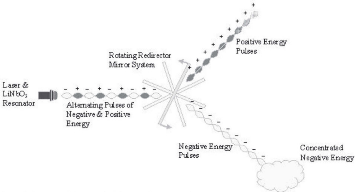
Figure 9. Conceptual Squeezed Light Negative Energy Generator
