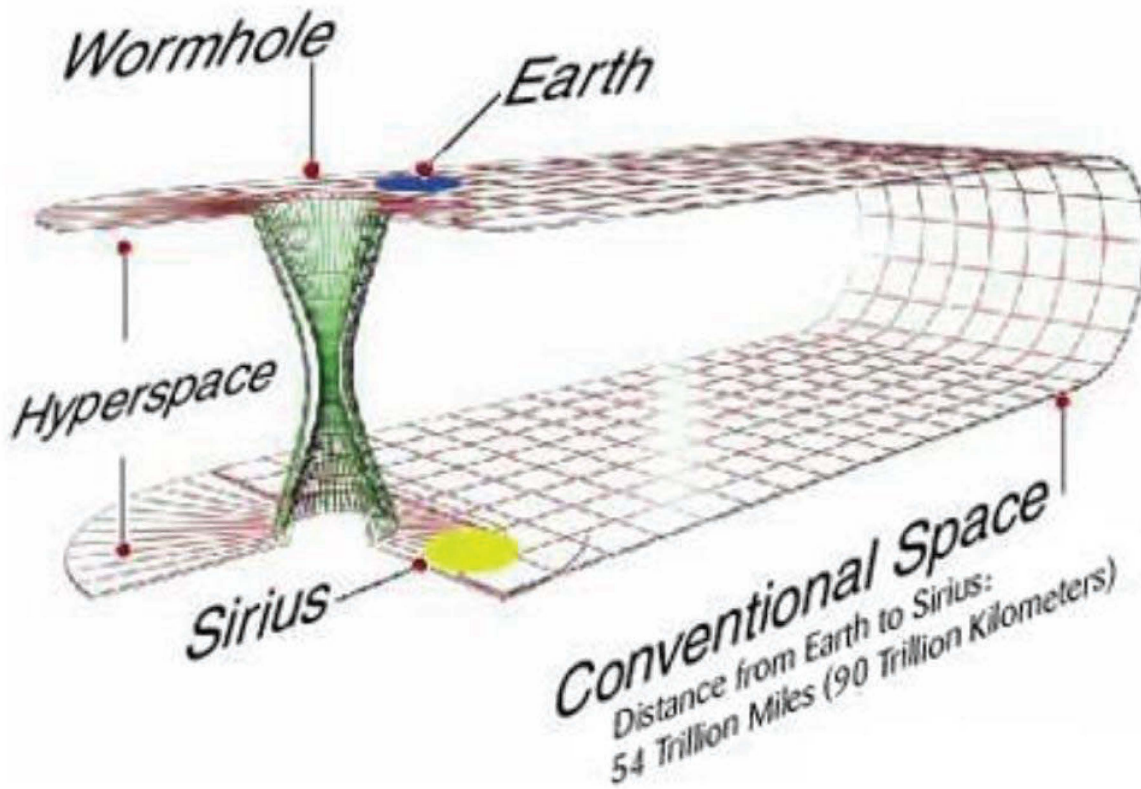
Figure 1. Intra-Universe Wormhole as a Hyperspace Shortcut Through Conventional Space
