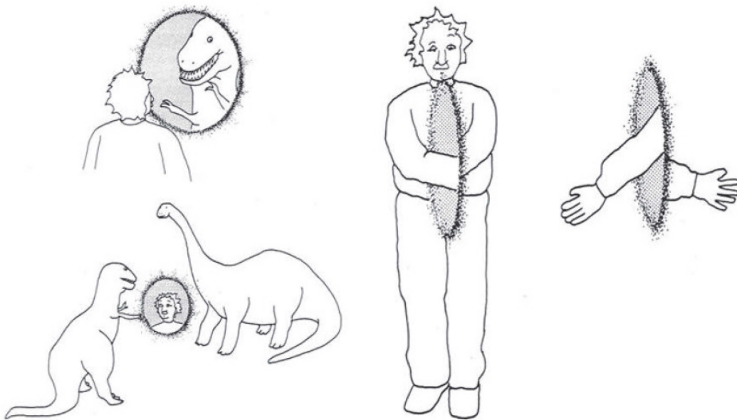
Figure 7. A Stargate (adapted from Reference 9)
