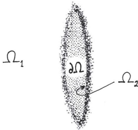
Figure 4. The Same Diagram as in Figure 3 Except as Viewed by an Observer Sitting in Region \Omega_1 Who Looks Through the Wormhole Throat \partial\Omega and Sees Remote Region \Omega_2 (dotted area inside the circle) on the Other Side
