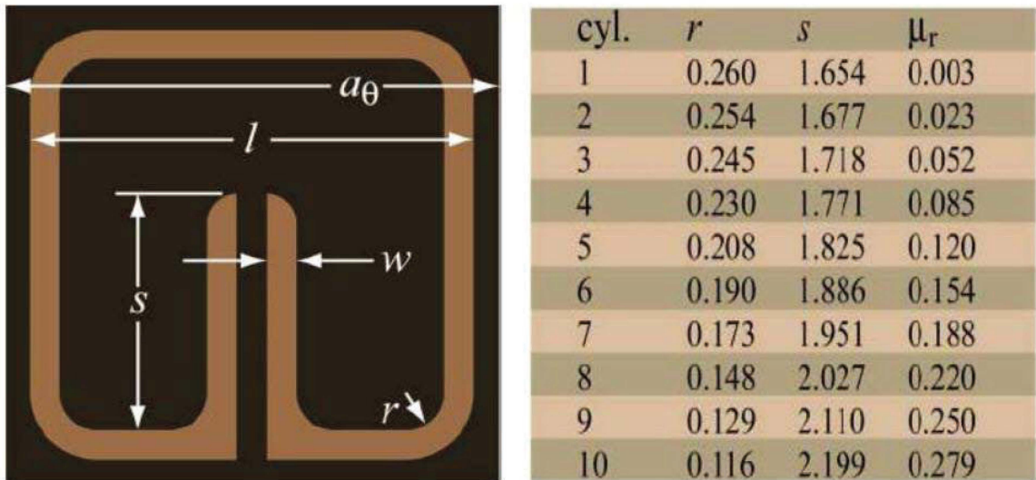
Figure 1. Example of a Metamaterial Component: The Magnetic Split Ring Resonator (SRR) Design. The in-plane lattice parameters are a_y = a_z = 10/3 mm. The ring is square, with edge length l = 3 mm and tracewidth w = 0.2 mm. The substrate is 381 \mu\text{m} -thick Duroid 5870 ( \epsilon = 2.33 , t_d = 0.0012 at 10 GHz, where t_d is the loss tangent). The Cu film, from which the SRRs are patterned, is 17 \mu\text{m} thick. The parameters r and s are given in the table together with the associated value of \mu_r . (Reference 6)
