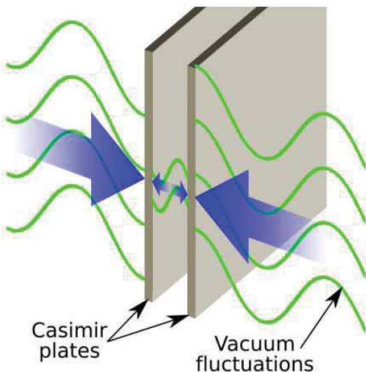
Figure 1. Illustration of the Casimir Effect
