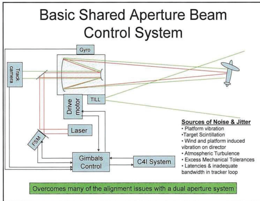
Figure 35. Basic Shared Aperture Beam Control System (TILL = Track Illuminator Laser; C4I = Command, Control, Computing, Communication & Intelligence equipment) (courtesy of the Directed Energy Professional Society).
