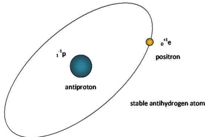
Figure 16. Antihydrogen Atom.
