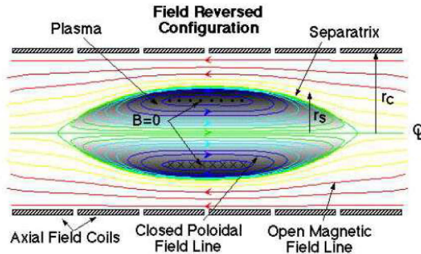
Figure 4. Field-Reversed Configuration
