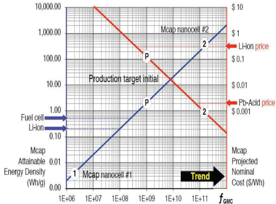
Figure 15. Specific Energy and Estimated Costs vs. f_{GMC}
