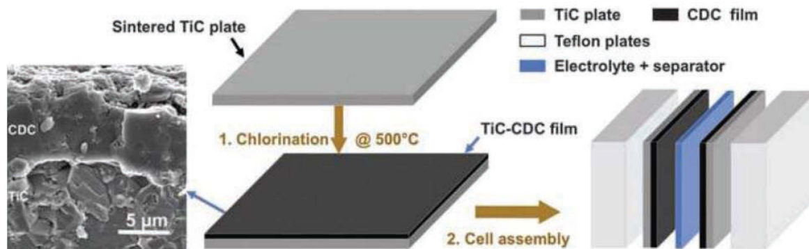
Figure 10. CDC Synthesis and Electrochemical Test Cell Preparation Schematic. 42
