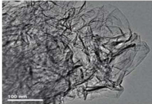
Figure 8. Transmission Electron Microscope Image of Graphene. This could be an excellent ultracapacitor electrode material with its high surface area and excellent conductivity. 33
