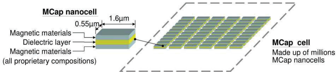
Figure 12. MCap Structure. MCap nanocell and MCap cell are fabricated using traditional semiconductor fabrication processes.
