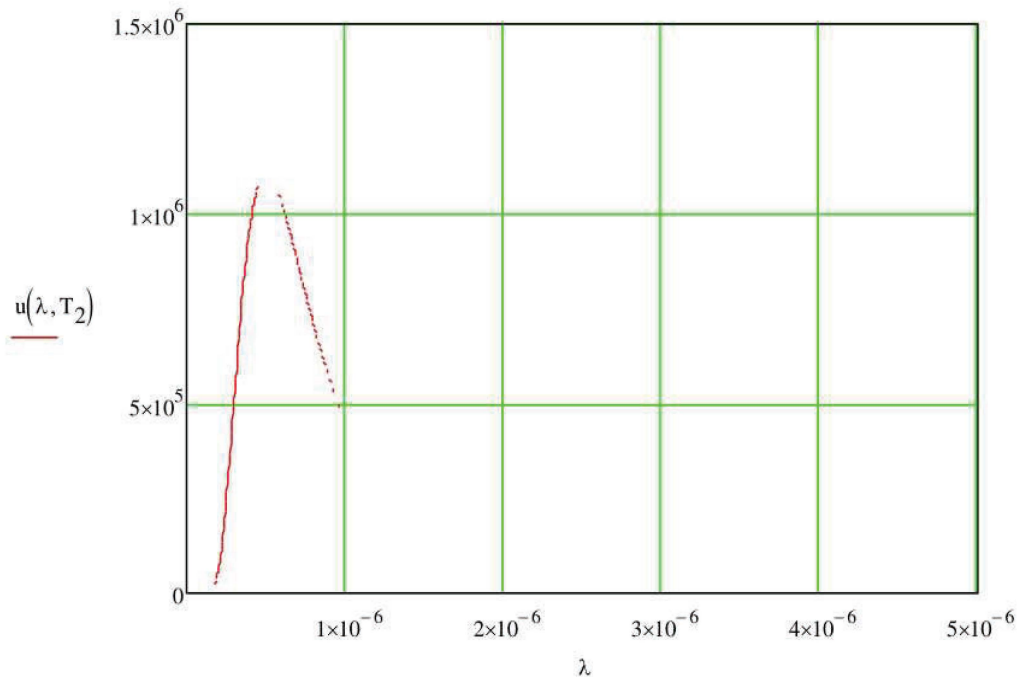
Figure 12. Energy Spectrum of the Sun at 5,778 K.
