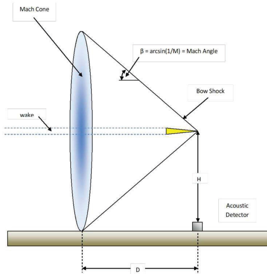
Figure 18. Mach Cone Generated by a Supersonic Object.
