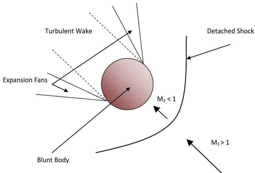
Figure 5. Supersonic Flow Past a Blunt Body (Spheroid).
