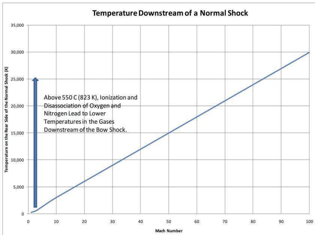
Figure 16. Peak Shock Layer Temperature for Hypersonic Objects.
