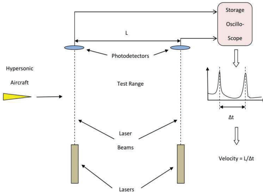
Figure 8. Laser-Based Chronograph.
