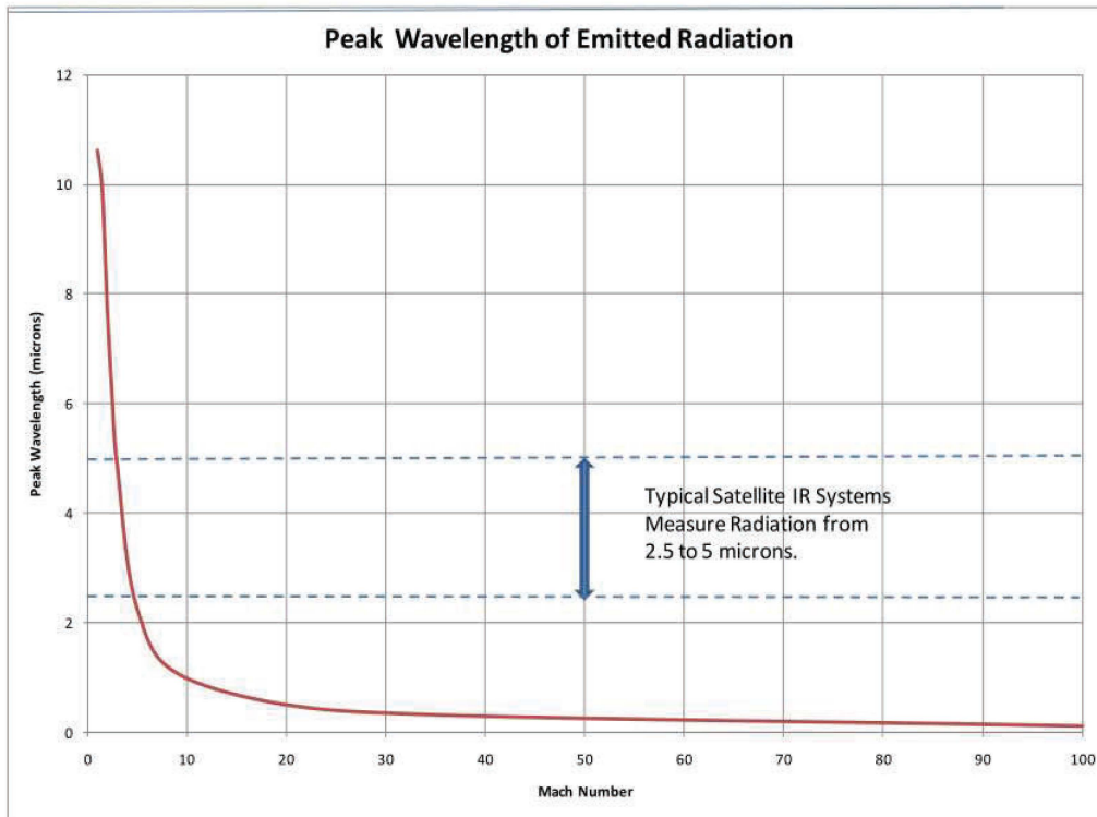
Figure 15. Peak Wavelength of the Infrared Radiation Emitted by Hypersonic Objects.
