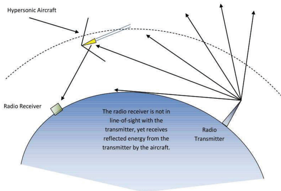
Figure 11. Radio Reflection Detector.
