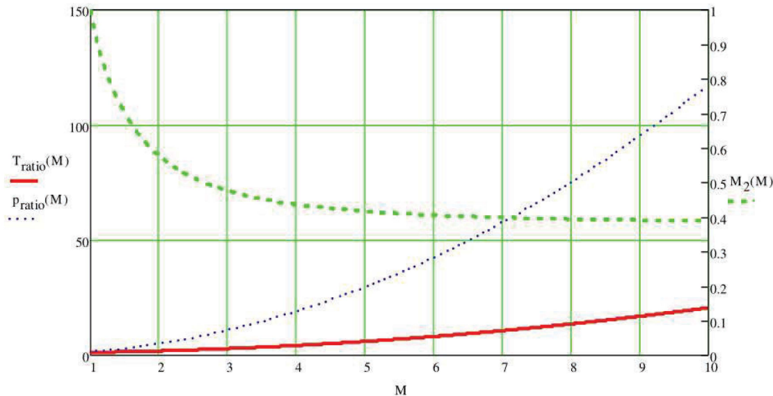
Figure 6. Ratios of Mach Number, Temperature, and Pressure Across a Normal Shock
