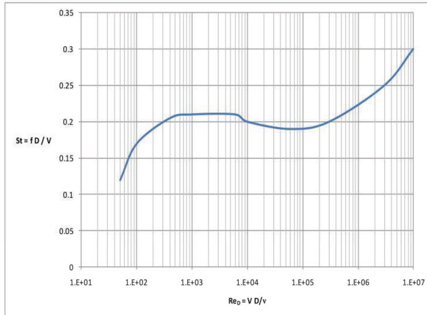
Figure 3. Strouhal Frequency as a Function of Reynolds Number for Flow Over a Circular Cylinder.
