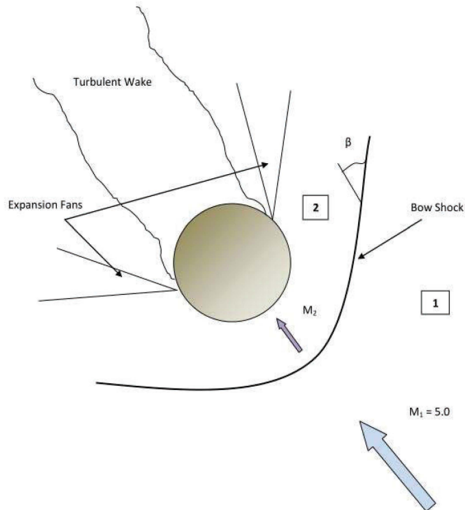
Figure 13. Hypersonic Flow Past a Sphere.
