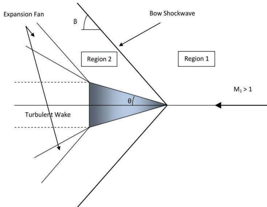
Figure 4. Supersonic Flow Past a Wedge-Shaped Body.
