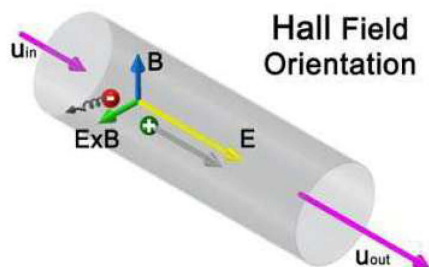
Figure 3. Field Orientation for Hall Field Systems and P5 Hall Thruster. Left: Figure shows the Hall field orientation. Right: P5 Hall Effect thruster being tested at the University of Michigan.
