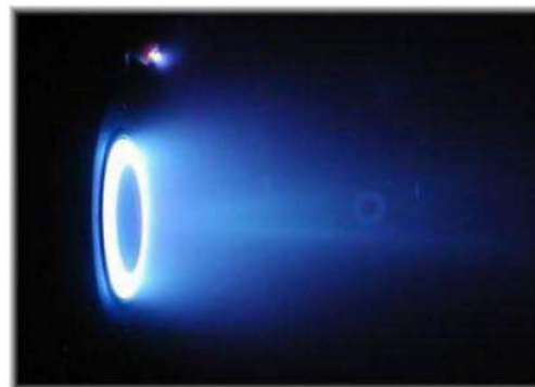
Figure 3. Field Orientation for Hall Field Systems and P5 Hall Thruster. Left: Figure shows the Hall field orientation. Right: P5 Hall Effect thruster being tested at the University of Michigan.
