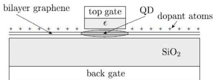
Figure 5. Quantum dot in bilayer graphene.
