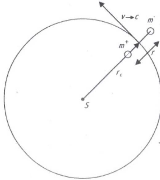
Figure 3. Circular motion of a pole-dipole particle.
