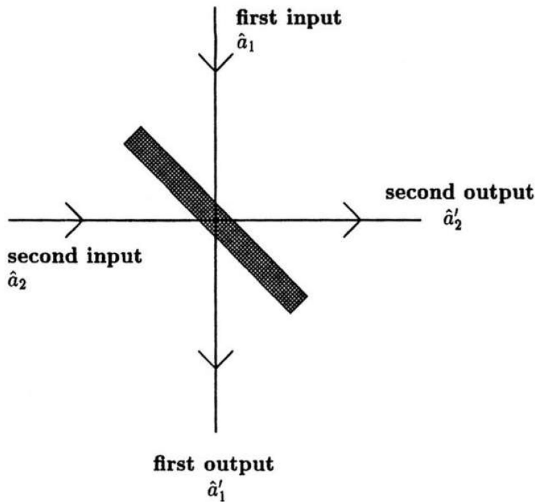
Figure 8. Schematic of an Ideal Lossless Beam Splitter. Two incident spatial-temporal light modes (with the annihilation operators \hat{a}_1 and \hat{a}_2 ) interfere optically to produce two emerging light modes (with the annihilation operators \hat{a}'_1 and \hat{a}'_2 ) (courtesy of Ulf Leonhardt).
