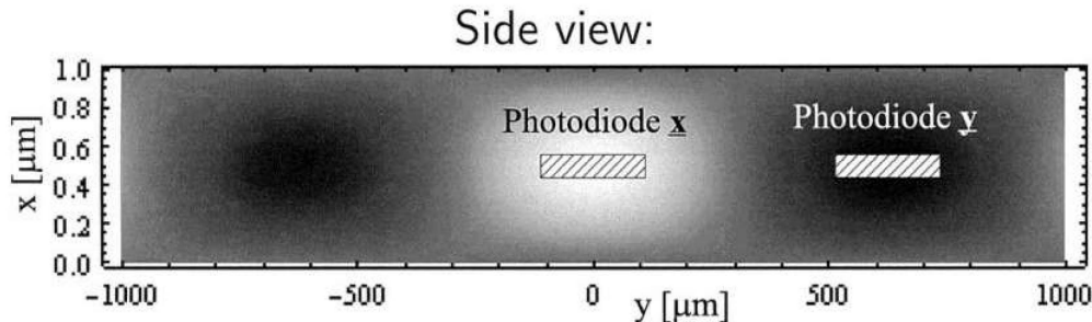
Figure 17. Experimental Setup of BHD Photodiodes and LO Field. (courtesy of P. Marecki) This setup is drawn on the plot of the y -component of the electric field of the TE1 mode of the Casimir cavity. The mode, serving as the LO, propagates in the z -direction perpendicular to the plot.
