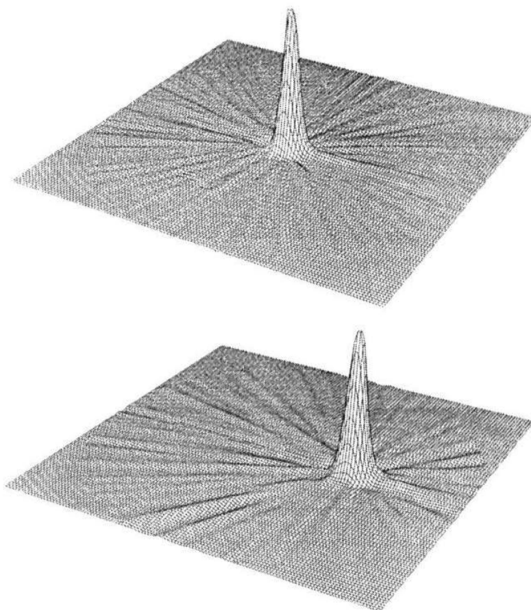
Figure 4. Wigner Function for a Vacuum (top) and for a Coherent State (bottom). This clearly shows that coherent states are just "displaced vacua" (Sect. IIB-3). Optical homodyne tomography was used to reconstruct the Wigner functions from experimental data (courtesy of Ulf Leonhardt).
