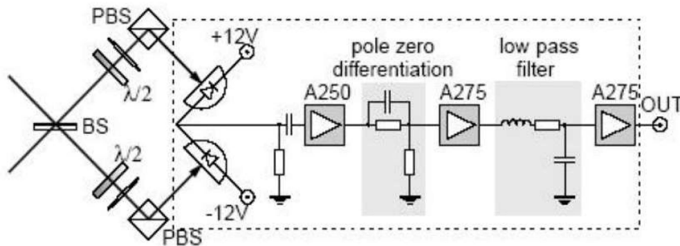
Figure 13. Time-Domain Balanced Homodyne Detector. (courtesy of P. Lodahl)
