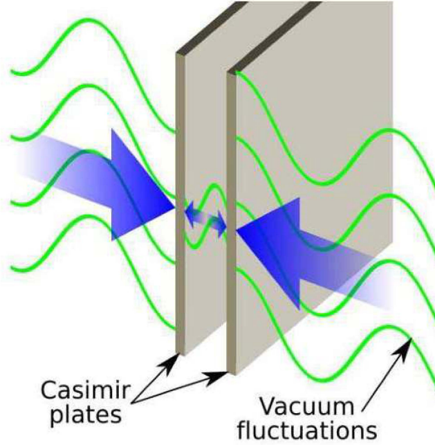
Figure 2. Schematic of the Casimir Effect.
