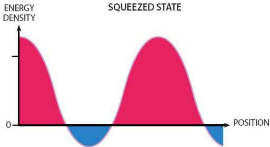
Figure 1. Illustration of a Squeezed State of Light. (courtesy of Lisa Burnett)
