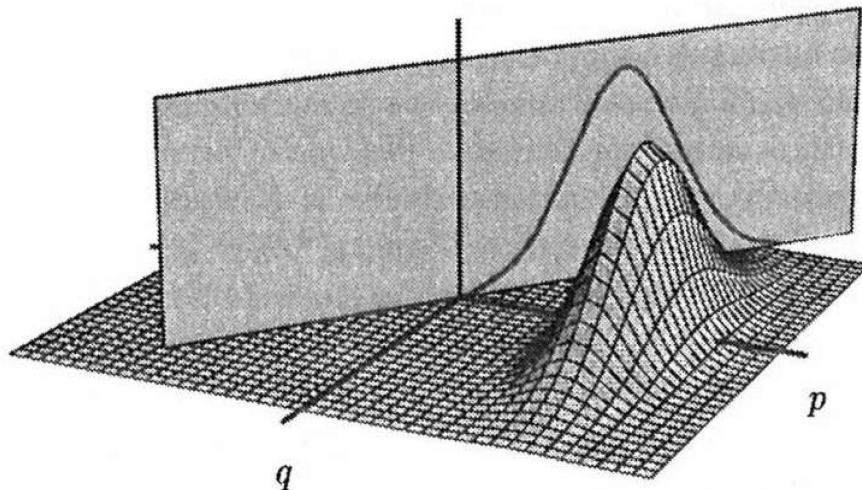
Figure 3. Illustration of Quantum Optical Homodyne Tomography (courtesy of Ulf Leonhardt). The Wigner function (3-dimensional hill on the right) is reconstructed in quantum phase space (gridded plane formed by quadratures q and p ) from its experimentally measured projections (curve in vertical 2-dimensional plane), which represents the scanning process of tomography. The vertical axis is the magnitude of the Wigner (quasiprobability) function.
