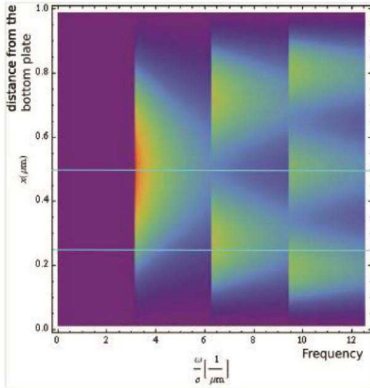
Figure 19. Predicted Casimir Spectral Density \sigma_{yy} . (courtesy of P. Marecki) \sigma_{yy} is related to the expected output of a BHD with the LO polarized along the y -direction (parallel to the plates) for the ground state in the Casimir cavity. This is plotted as a function of the position x \in [0, a] between the plates (separation a = 1 \mu\text{m} is assumed) and the frequency \omega \in [0, 4\pi c/a] . Negative values (suppression of fluctuations) are shown in deep purple.
