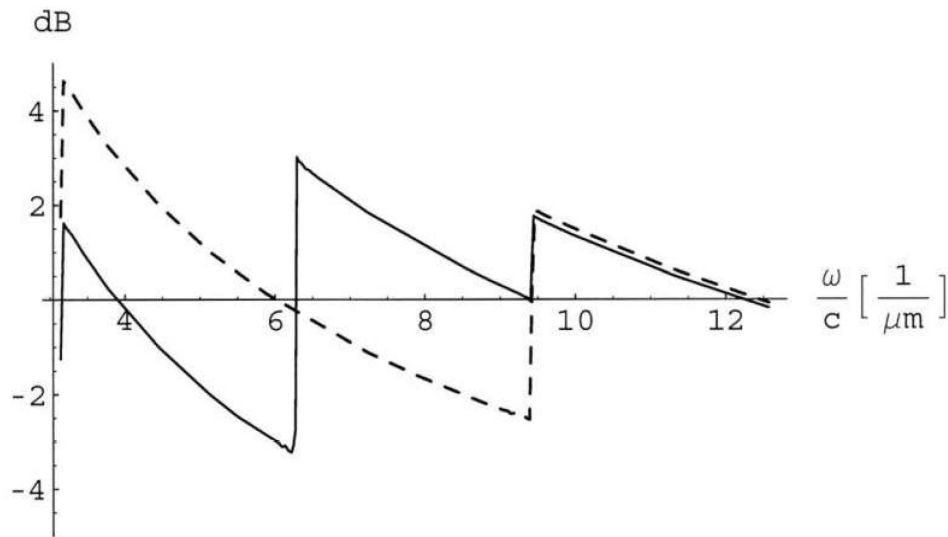
Figure 20. Predicted Suppression of Vacuum Fluctuations in dB. (courtesy of P. Marecki) Vacuum fluctuations in the ground state (for field operators restricted to the frequency \omega ) relative to vacuum fluctuations (in the absence of the plates) for a BHD at x = 0.25 \mu\text{m} (solid line) and x = 0.5 \mu\text{m} (dashed line) within the cavity. The frequency range is \omega \in [0, 4\pi c/a] .
